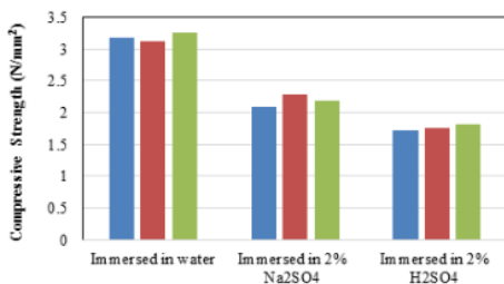
Fig 6. Compressive strength of geopolymer mortar
