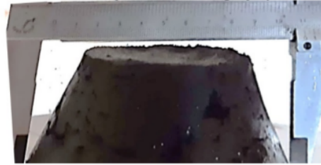
Fig 2. The flow of fresh mortar geopolymer
